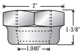
No. 15 Taper Bore read: 1-13/32" -10
