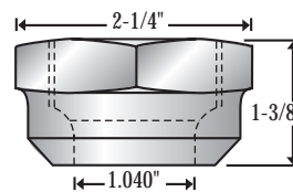
No. 55 Taper Bore read: 1-9/16" -12
